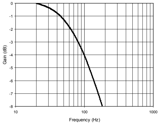
HAH1BV S/18 Frequency Bandwidth
