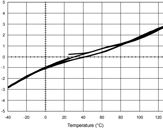
HAH1BV S/18 Gain Error (%)
