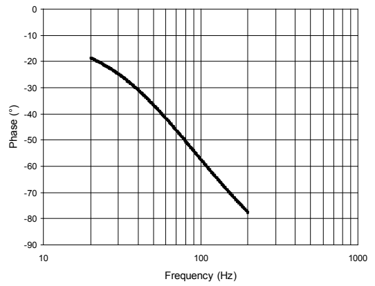
HAH1BV S/18 Phase
