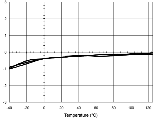
HAH1BV S/18 Electrical offset Error (A)
